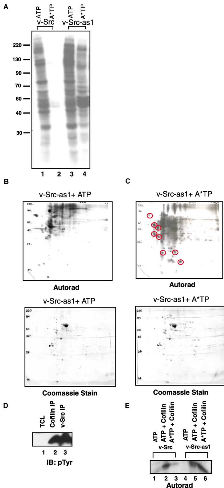
Figure 1. Differential Phosphorylation of Direct v-Src Substrates in v-Src-as1 NIH 3T3 Cell Lysate with [\gamma\text{-}^{32}\text{P}]\text{N}^6(\text{Benzyl})\text{ATP}
